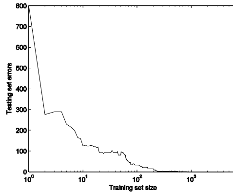
Figure 1: SVM Misclassification Rate
